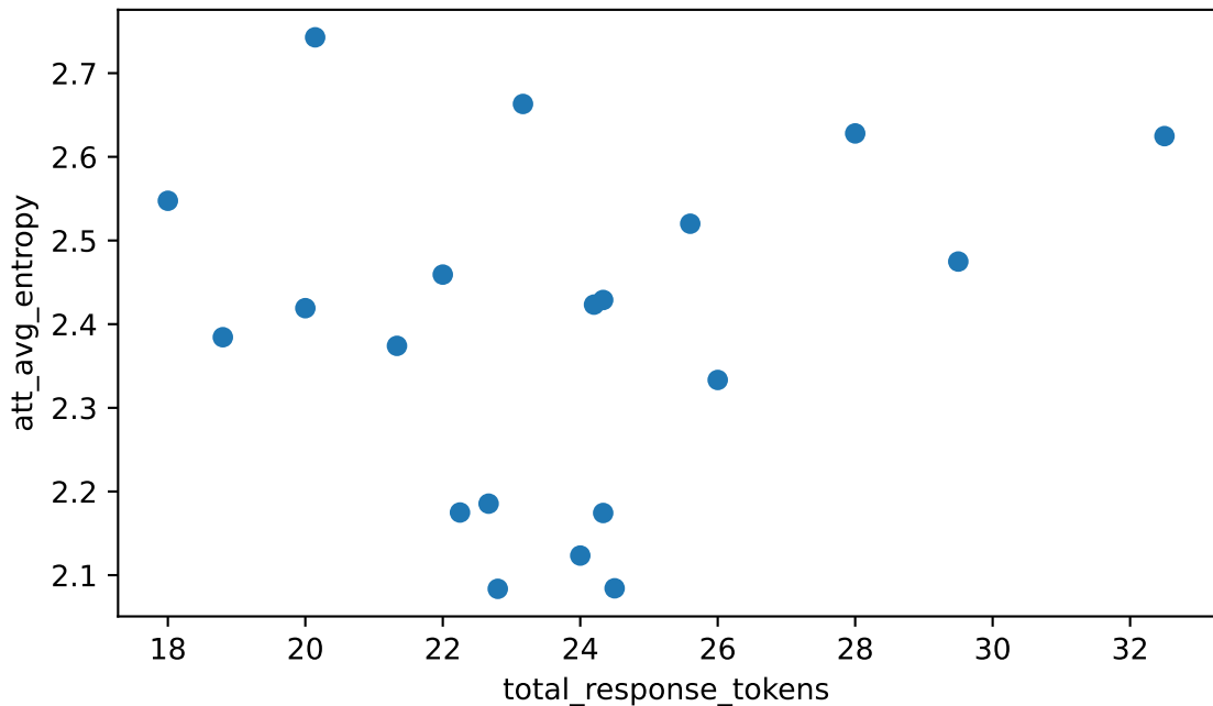
total_response_tokens vs att_avg_entropy Spearman rho=+0.059 (weak), n=20
