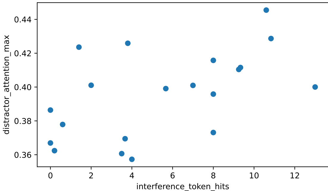
interference_token_hits vs distractor_attention_max Spearman rho=+0.523 (moderate), n=20
