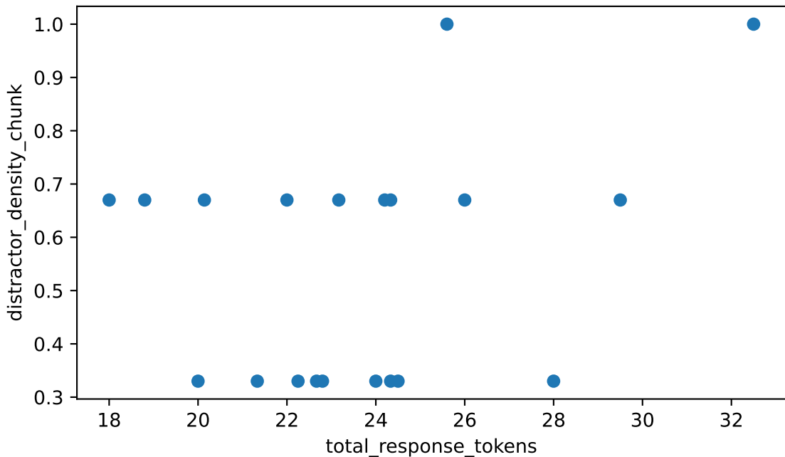
total_response_tokens vs distractor_density_chunk Spearman rho=+0.212 (weak), n=20
