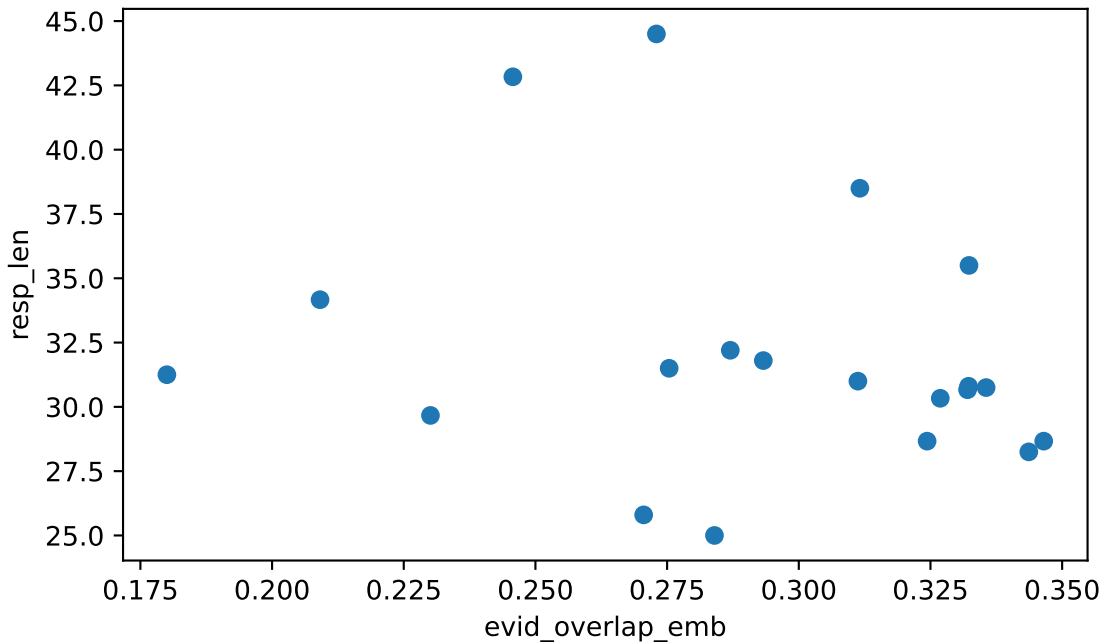
evid_overlap_emb vs resp_len Spearman rho=-0.288 (weak), n=20
