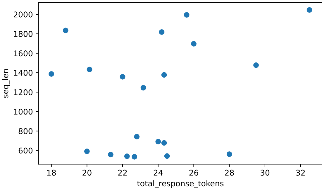
total_response_tokens vs seq_len Spearman rho=+0.228 (weak), n=20
