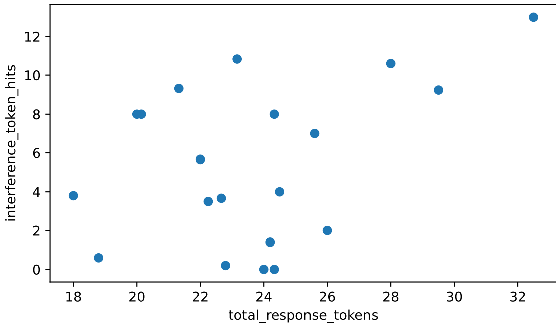
total_response_tokens vs interference_token_hits Spearman rho=+0.224 (weak), n=20
