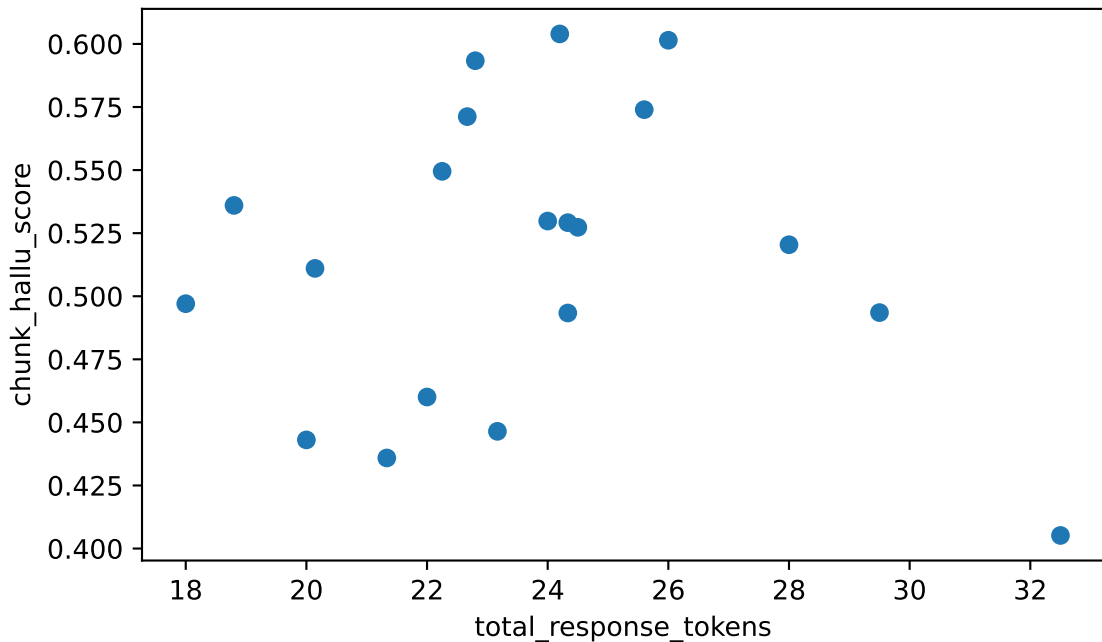
total_response_tokens vs chunk_hallu_score Spearman \rho =+0.105 (weak), n=20
