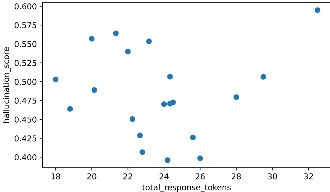
total_response_tokens vs hallucination_score Spearman rho=-0.105 (weak), n=20
