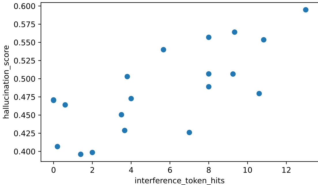
interference_token_hits vs hallucination_score Spearman rho=+0.747 (strong), n=20
