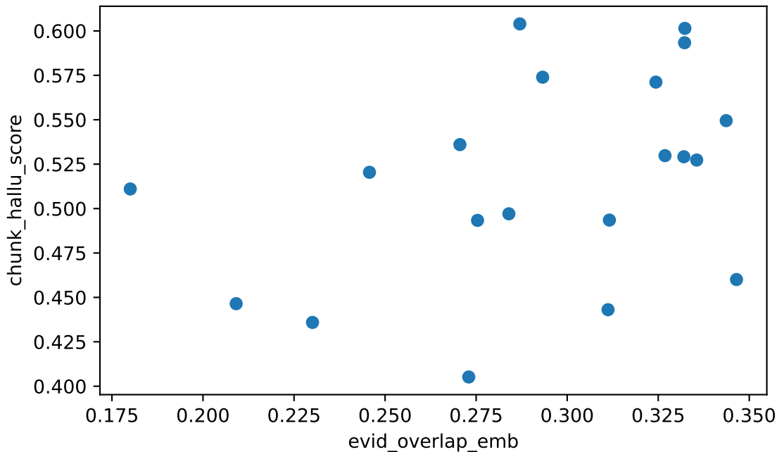
evid_overlap_emb vs chunk_hallu_score Spearman rho=+0.408 (moderate), n=20
