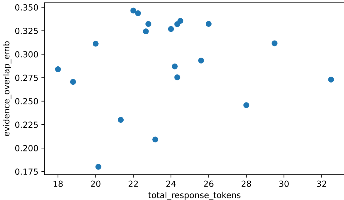
total_response_tokens vs evidence_overlap_emb Spearman rho=+0.126 (weak), n=20
