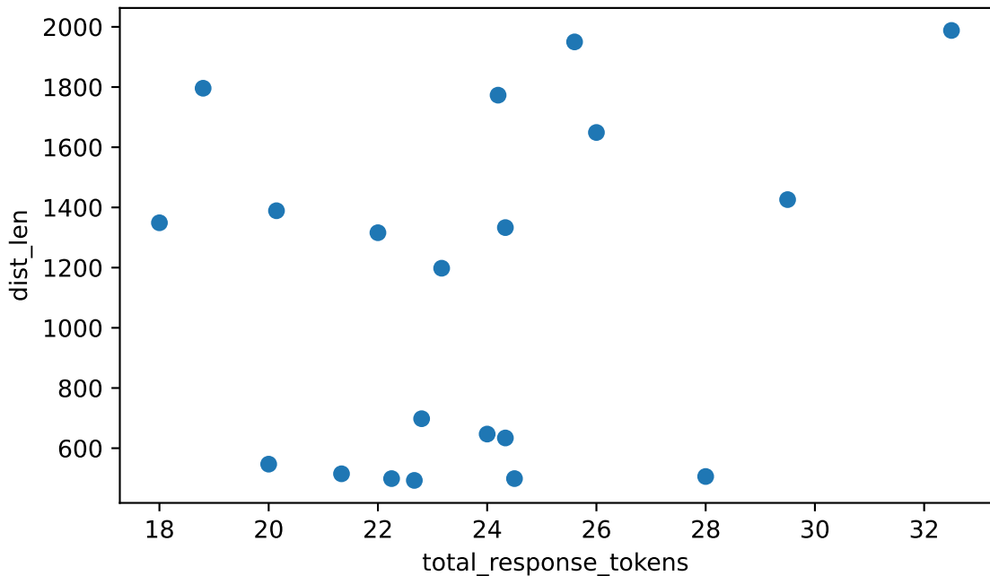
total_response_tokens vs dist_len Spearman rho=+0.202 (weak), n=20
