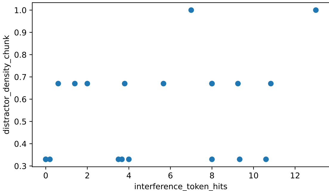
interference_token_hits vs distractor_density_chunk Spearman rho=+0.318 (weak), n=20
