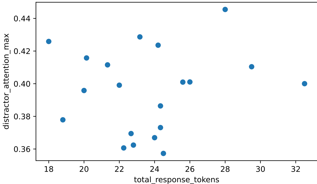
total_response_tokens vs distractor_attention_max Spearman rho=+0.053 (weak), n=20
