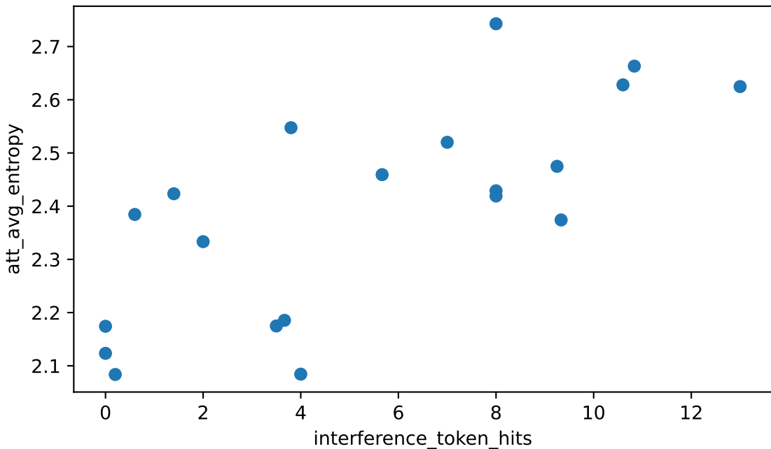
interference_token_hits vs att_avg_entropy Spearman rho=+0.730 (strong), n=20
