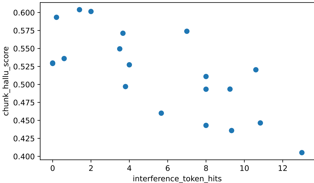
interference_token_hits vs chunk_hallu_score Spearman rho=-0.747 (strong), n=20
